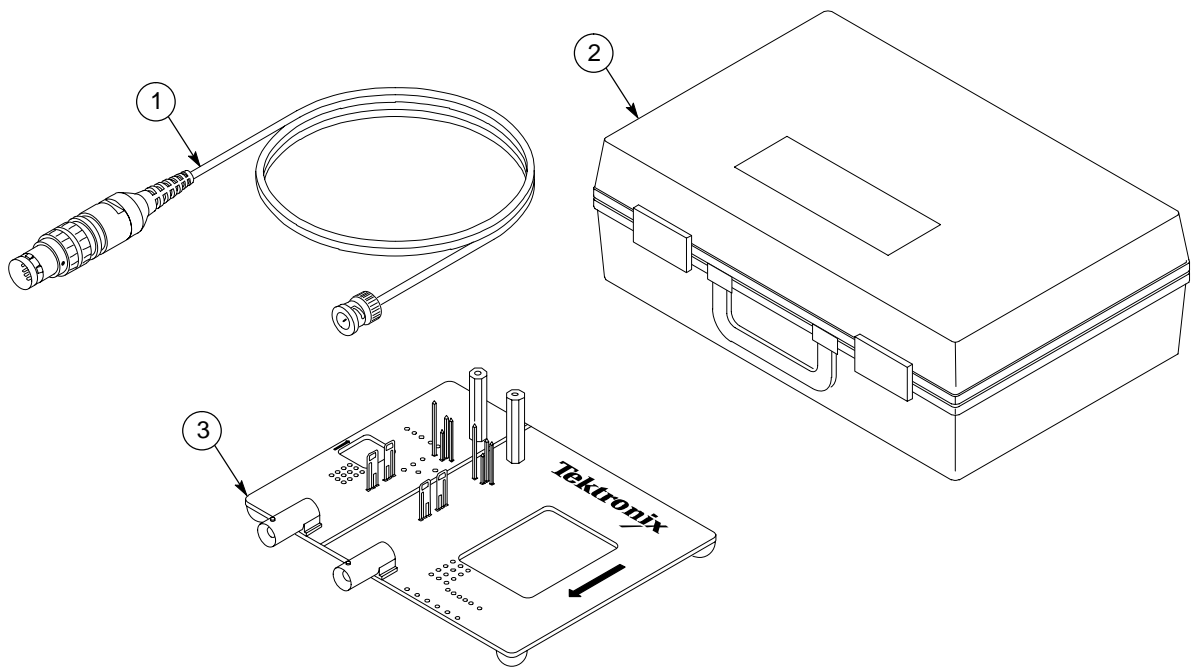
Figure 8-3: TCPA300 and TCPA400 optional accessories
